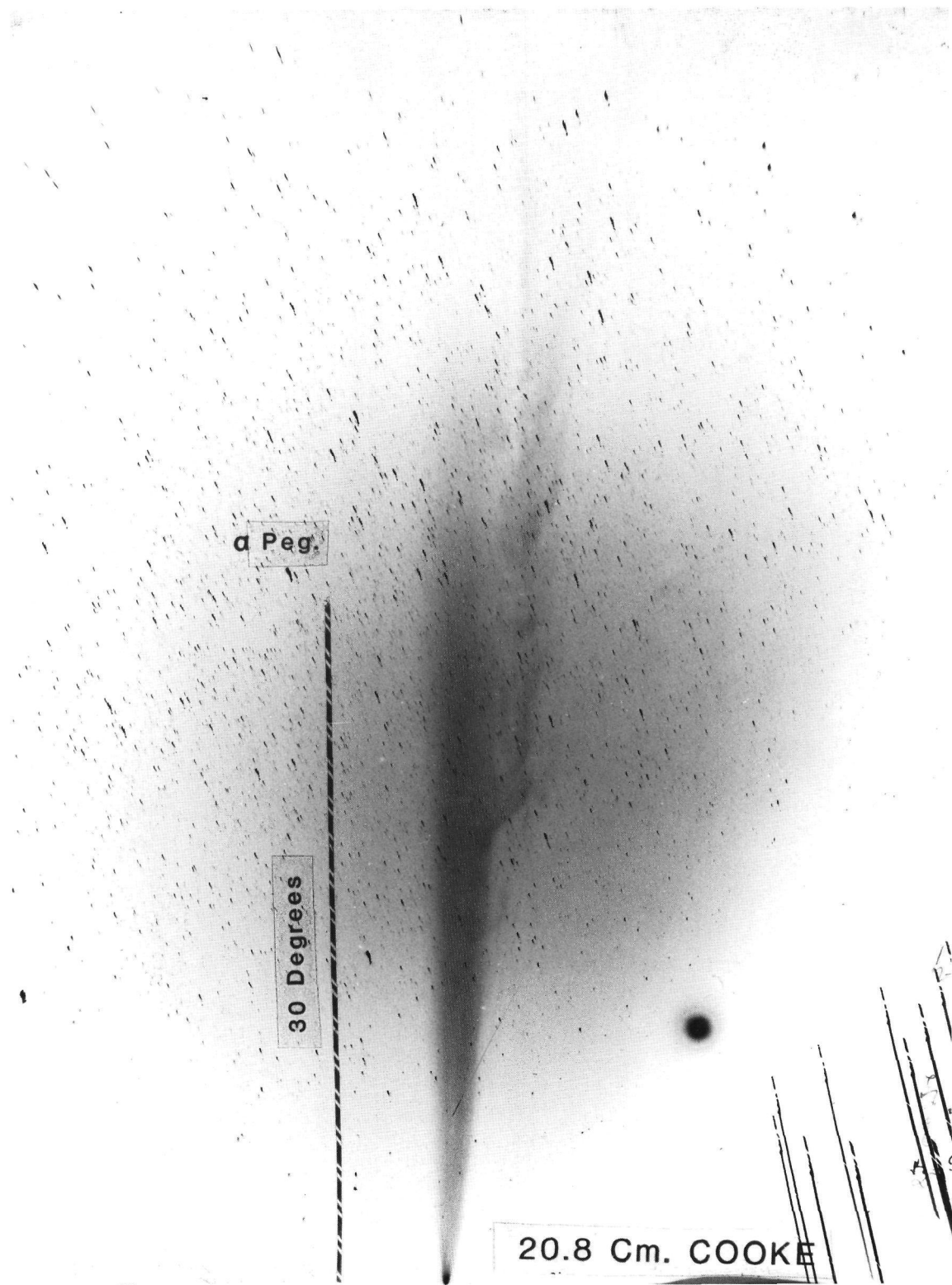
Figure 5. Photograph of Comet Halley obtained on May 13, 1910.
